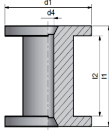
Graph. 5 Cylindrical spool
